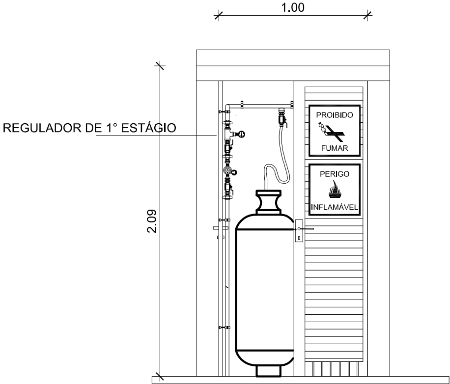
VISTA FRONTAL
